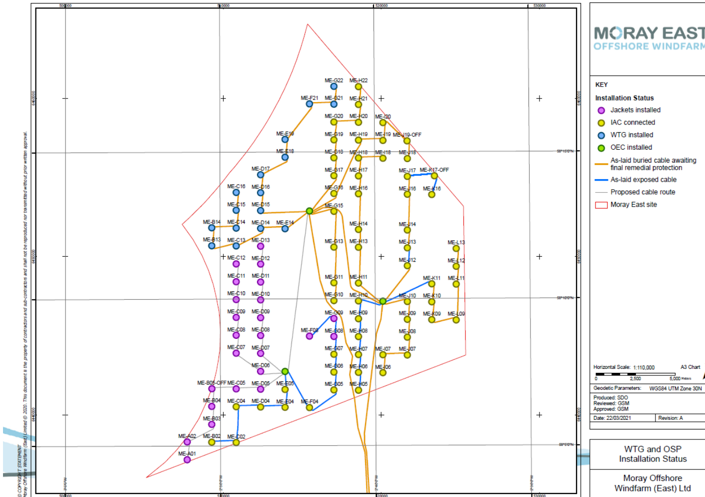
Figure 1. Moray East Offshore Windfarm
