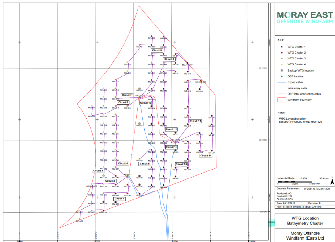
Figure 1: Location of Wind Farm Site
